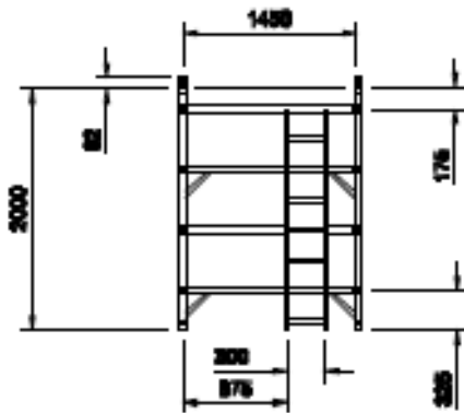
2m 4-Rung
