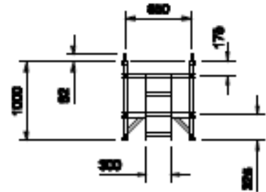
1m 2-Rung
