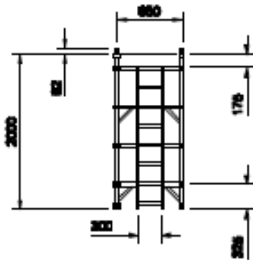
2m 4-Rung
