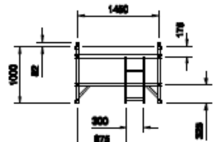
1m 2-Rung
